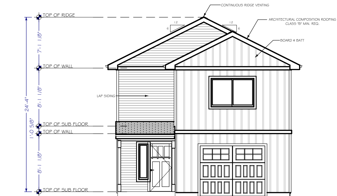
FRONT ELEVATION
