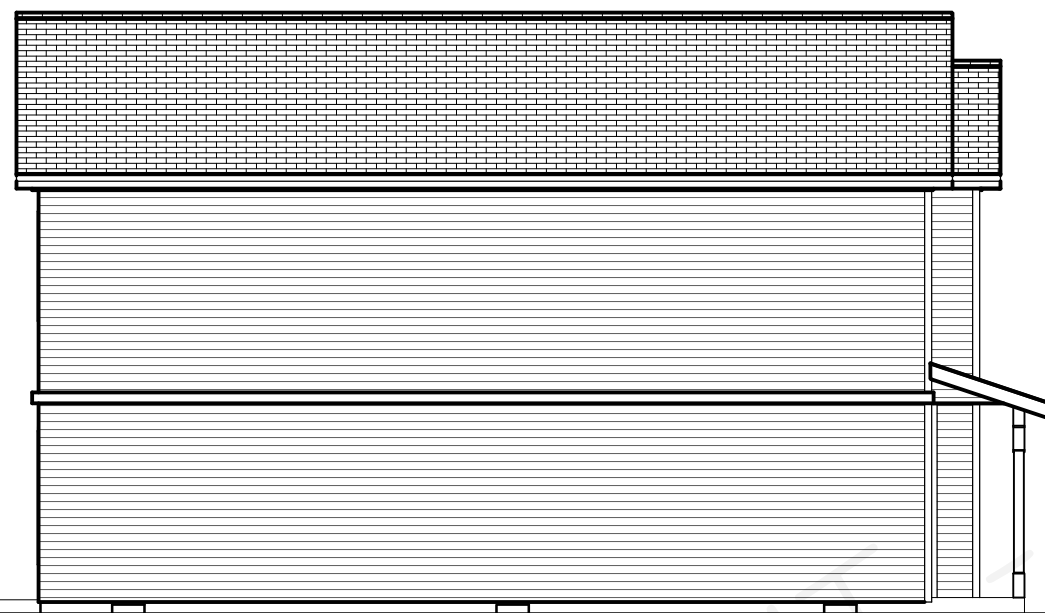
LEFT ELEVATION
